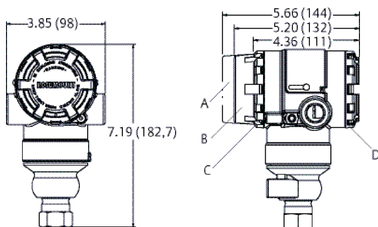
Illustration 13 : Rosemount 2051T
